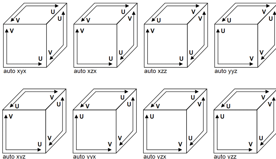
Abbildung 2: Quader-Mapping
