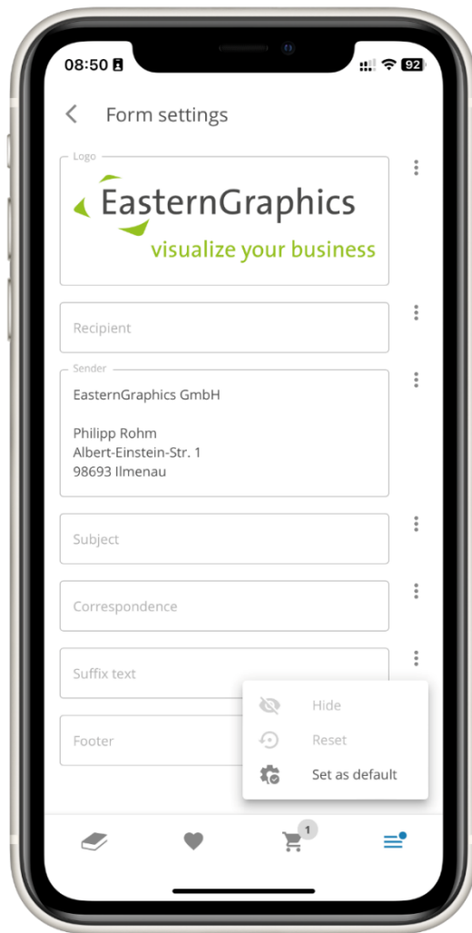
Figure 1 - Formulareinstellungen
